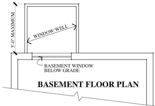
ILLUSTRATION E (BUILDING HEIGHT/FINISH GRADE-WINDOW WELLS)
