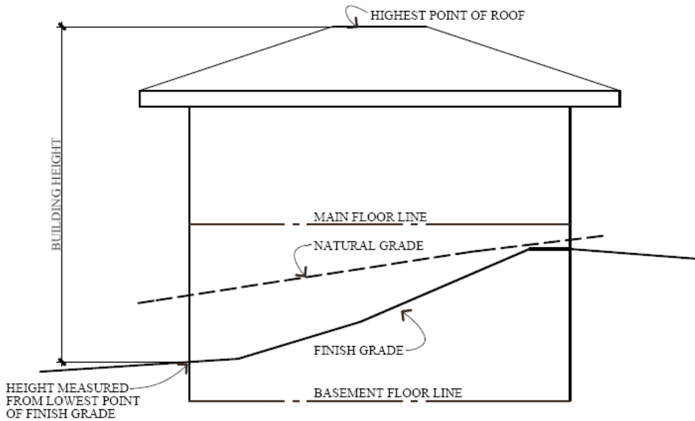
ILLUSTRATION C2 (BUILDING HEIGHT/FINISH GRADE- FINISH AND NATURAL GRADES)
