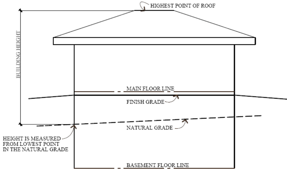
ILLUSTRATION C1 (BUILDING HEIGHT/FINISH GRADE- FINISH AND NATURAL GRADES)
